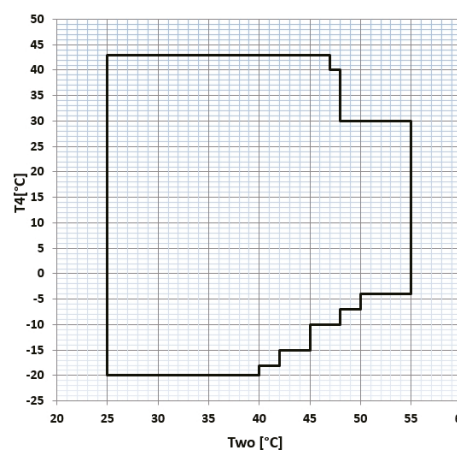
Heating mode
